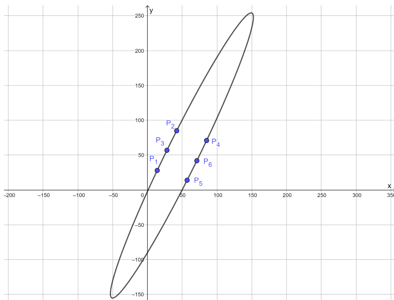
Slika 2. Elipsa kroz (14, 28), (42, 85), (28, 57), (85, 71), (57, 14), (71, 42)
