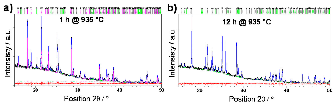
Figure 2. Rietveld refinements of the bulk glass samples crystallized for (a) 1 h and (b) 12 h at 935 °C. Experimental data are given by black line, the calculated pattern is shown in blue, while the red line represents the difference curve. Grey vertical marks show the positions of diffraction lines belonging to monoclinic W_2O_3(PO_4)_2 phase, magenta bars represent reflection of orthorhombic W_2O_3(PO_4)_2 phase, while the positions of WO_3 lines are given as green vertical marks.
