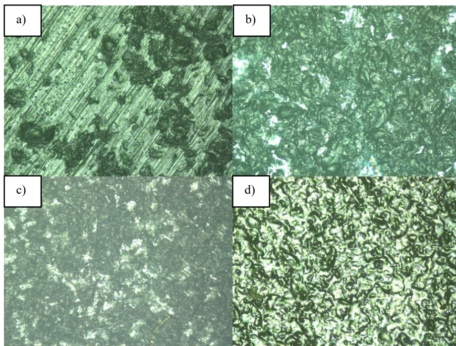
Figure 4. Optical images (×100) of the non-aged samples (a) LS10, (b) LS11, (c) LS20, and (d) LS21. Material processing is visible only for LS10 (a).
