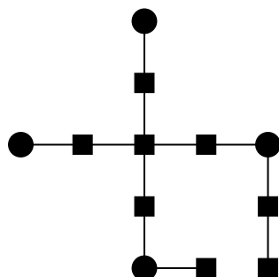
(e) T
