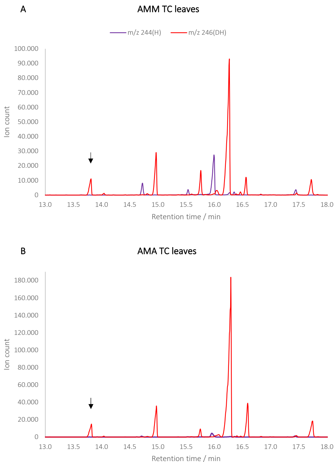
Figure 12. Ion abundance chromatogram from GC–MS analysis of sesquiterpene lactones helenalin (H, m/z 244) and dihydrohelenalin (DH, m/z 246) from Arnica montana ssp. montana (A) and atlantica (B) leaf extracts from nine plants grown in tissue culture conditions. Internal standard \alpha -santonin peak (m/z 246) is marked by an arrow.
