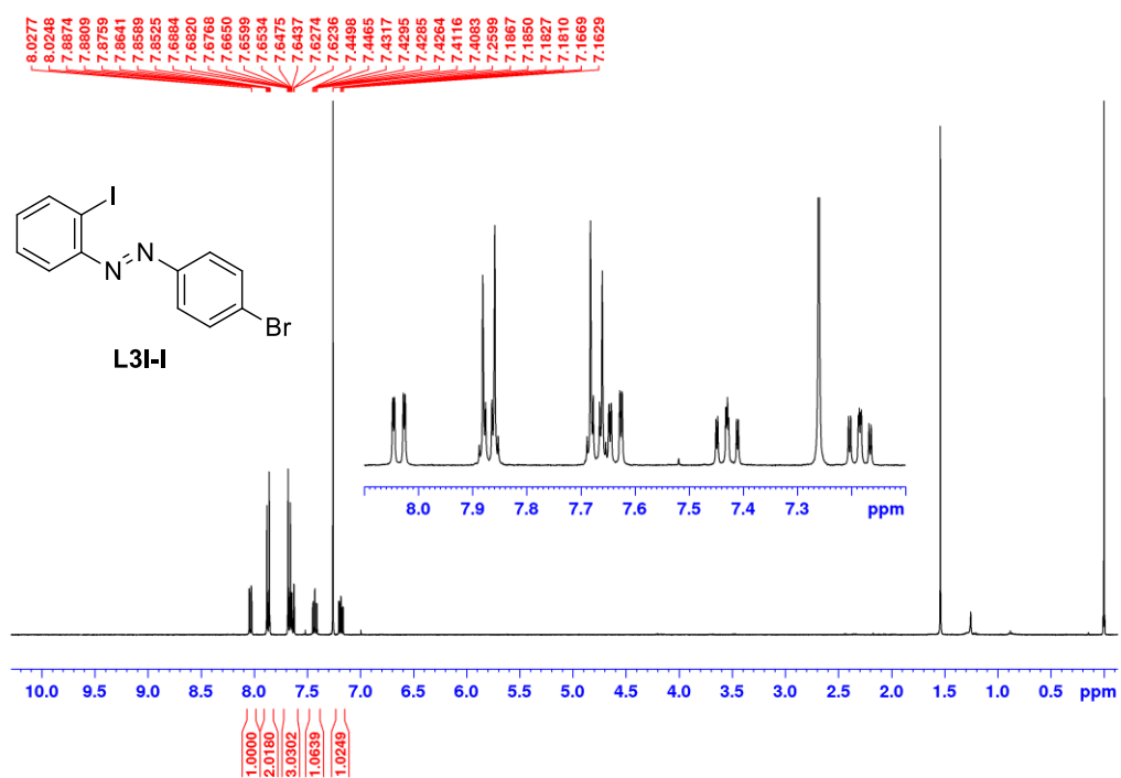
Slika D90. ^1\text{H} NMR spektar L3I-I u \text{CDCl}_3 (400 MHz).
