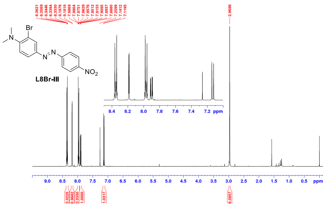
Slika D152. ^1\text{H} NMR spektar L8Br-III u \text{CDCl}_3 (400 MHz).
