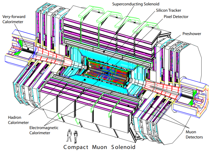
Figure 2.5: The cross section view of the CMS detector showing its main subdetector systems. Figure taken from [45]
