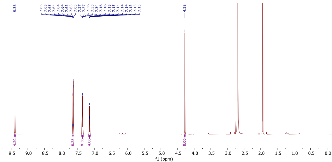
Slika D30. ^1\text{H} NMR spektar K10 , \text{CD}_3\text{CN} , 600 MHz, -40\text{ }^\circ\text{C} .
