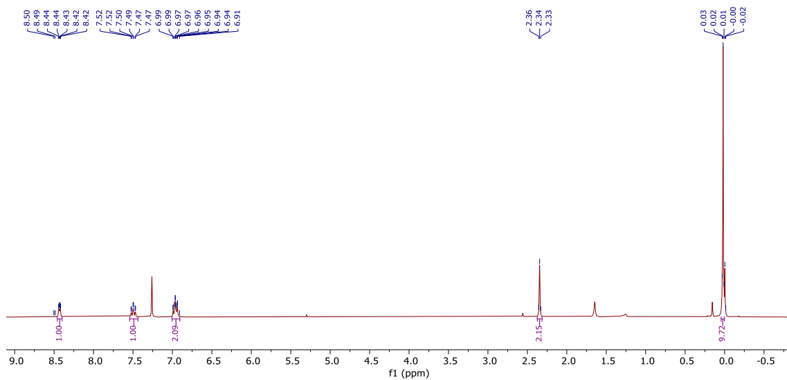
Slika D25. ^1\text{H} NMR spektar L7a , \text{CDCl}_3 , 300 MHz, 25 °C.
