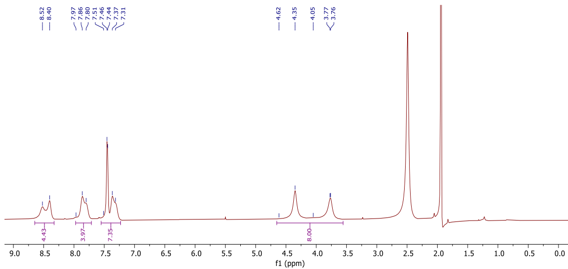
Slika D28. ^1\text{H} NMR spektar K6 , \text{CD}_3\text{CN} , 600 MHz, -40\text{ }^\circ\text{C} .
