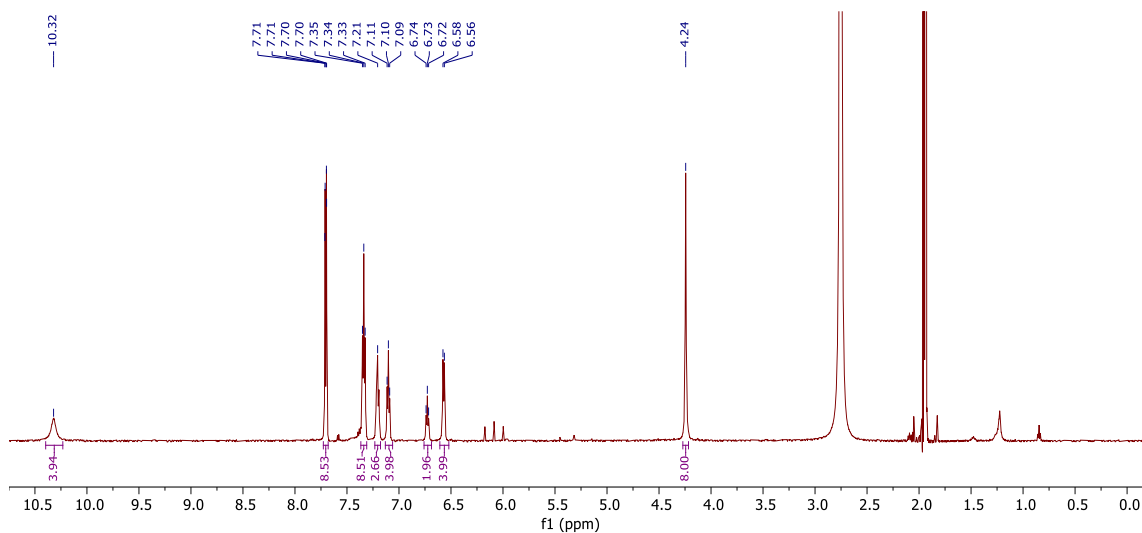
Slika D29. ^1\text{H} NMR spektar K8 , \text{CD}_3\text{CN} , 600 MHz, -40\text{ }^\circ\text{C} .
