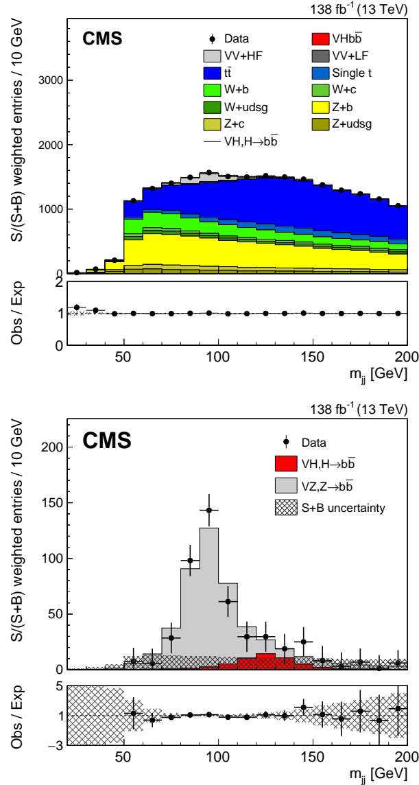
Figure 5.2: Dijet invariant mass distributions, combining all channels and data-taking periods, with events weighted according to S/(S+B) . The distributions are evaluated after the fit to data and as a result, the fitted signal strength is utilized to scale the signal component. To display the invariant mass peaks of the VZ(Z \rightarrow b\bar{b}) and VH(H \rightarrow b\bar{b}) resonances, all background processes other than the VH and VZ contributions are also exhibited (top) or subtracted (bottom).
