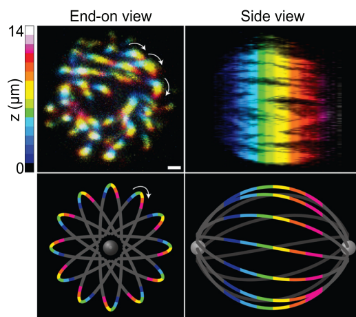
FIGURE 1 End-on view and side view of a human mitotic spindle. ( Top ) Projections of confocal images, color coded for the position along the pole-to-pole axis (see color bar ), of the metaphase spindle in a live HeLa cell expressing PRC1-GFP shown in the end-on view ( left ) and side view ( right ). Scale bars, 1 \mu\text{m} . ( Bottom ) Schematic representations of spindle microtubule bundles shown in the end-on view ( left ) and side view ( right ). The arrows show the direction of the bundle twist along the pole-to-pole axis when looking toward the observer. The clockwise direction of the arrows indicates left-handed twist. To see this figure in color, go online.
