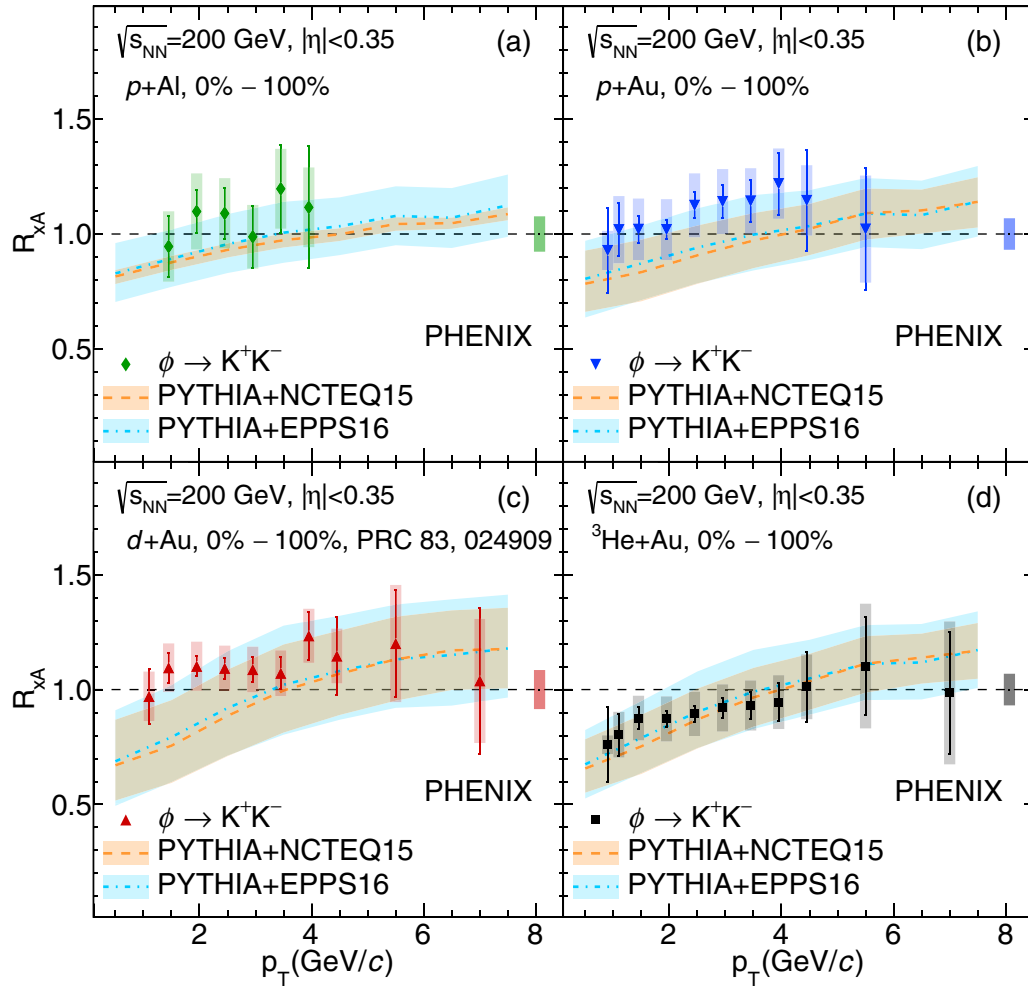
FIG. 6. Experimental results on \phi -meson production in (a) p + \text{Al} , (b) p + \text{Au} , (c) d + \text{Au} [2], and (d) {}^3\text{He} + \text{Au} collisions at \sqrt{s_{\text{NN}}} = 200 GeV at midrapidity ( |\eta| < 0.35 ) and comparisons to EPPS16 [33] and NCTEQ15 [34] nuclear PDF calculations.
