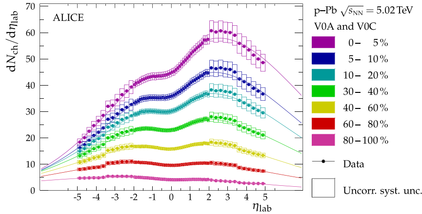
Fig. 2. Charged-particle pseudorapidity density in p-Pb collisions at \sqrt{s_{NN}} = 5.02 TeV in seven centrality classes based on the V0A and V0C estimators. The lines are obtained using a fit of a scaled, normal distribution in rapidity Eq. (2) to the data (discussed in Section 4).
