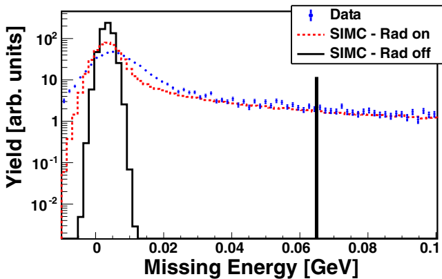
FIG. 4. Hydrogen missing energy spectra for Q^2 = 8 ( \text{GeV}/c ) 2 comparing data (blue dots) and Monte Carlo with (red dashed line) and without (black line) radiative correction. The vertical black line at 65 MeV indicates the E_{\text{miss}} cut for hydrogen.
