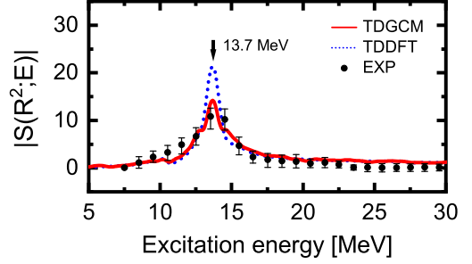
FIG. 2. The experimental ISGMR strength function in ^{208}\text{Pb} [30], in units of 10^3 \text{ fm}^4/\text{MeV} , compared with the results of the TD-DFT and TD-GCM (four basis trajectories) calculations. See text for description.
