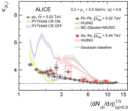
Fig. 5. Kurtosis \kappa_{(p_T)} shown as a function of \langle dN_{ch}/d\eta \rangle_{|\eta|<0.5}^{1/3} in Pb–Pb collisions at \sqrt{s_{NN}} = 5.02 TeV, Xe–Xe collisions at \sqrt{s_{NN}} = 5.44 TeV and pp collisions at \sqrt{s} = 5.02 TeV. The predictions from different event generators and hydrodynamic calculations from MC-Glauber+MUSIC model [40,41] are represented by colored bands. The dashed line indicates the Gaussian baseline. The statistical (systematic) uncertainties are represented by vertical bars (boxes).
