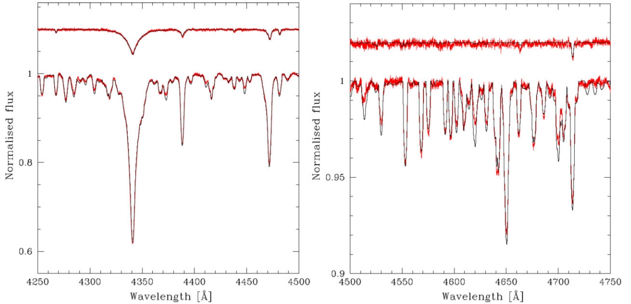
Figure 13. Optimal fitting of disentangled spectra for the primary component (lower) and secondary component (upper). Disentangled spectra are in red, optimal fits in black. The region of the spectra centred on the H \gamma line (left panel) and various metal lines in the spectral range from \lambda 4500 to 4750 Å (right panel) are shown.
