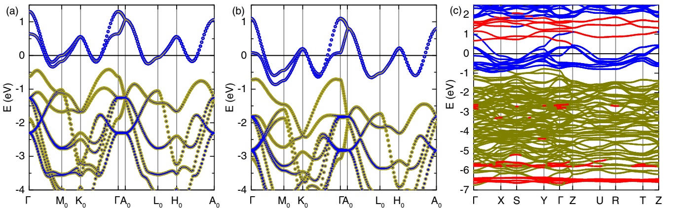
FIG. 12. (a) DFT-calculated electronic bands of 2\text{H-NbS}_2 with DFT-relaxed lattice parameters. (b) DFT-calculated electronic bands of 2\text{H-NbS}_2 with additional 2/3 electrons per Nb atom and the lattice parameters borrowed from DFT-relaxed \text{Co}_{1/3}\text{NbS}_2 structure. Blue and yellow colors reflect the relative weights of niobium and sulfur orbitals in particular states. (c) DFT-calculated electronic bands of \text{Co}_{1/3}\text{NbS}_2 in antiferromagnetically ordered state. The colors mark the dominant character of electronic states: blue indicates that the electronic state is predominantly composed of niobium orbitals, yellow represents the dominance of sulfur orbitals, and red specifies the dominance of cobalt orbitals in the electronic state.
