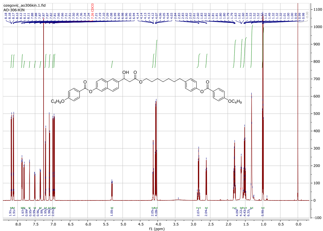
D1.15. 1 H NMR spektar spoja BN-7-BB, (S)-BN-7-BB
