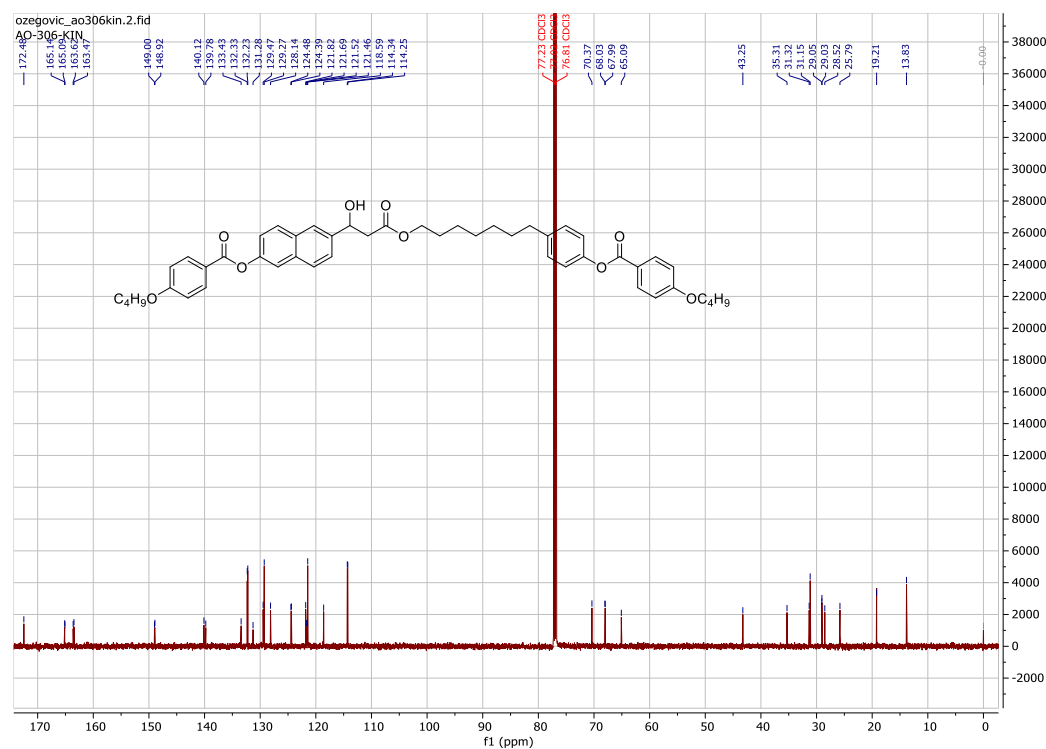
D1.16. 13 C NMR spektar spoja BN-7-BB, (S)-BN-7-BB
