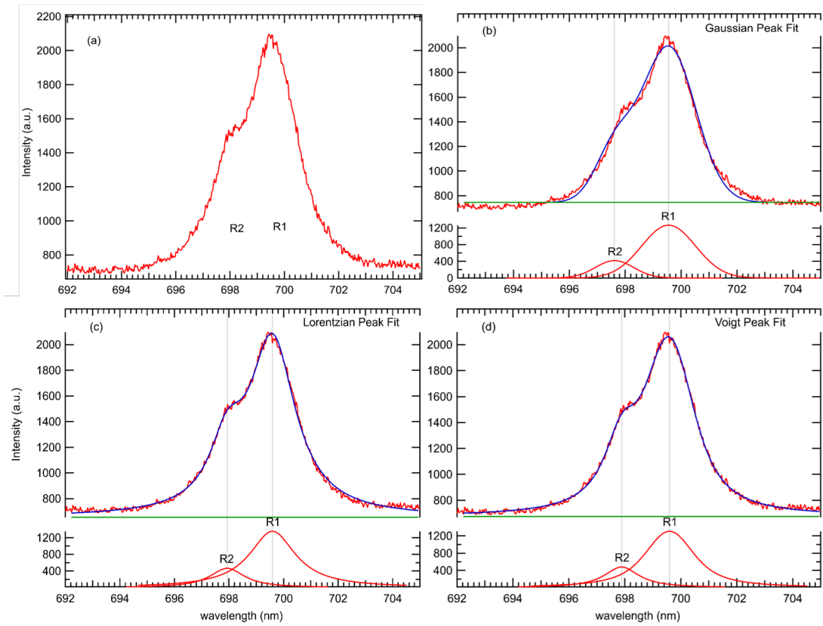
Figure A.2: (a) Ruby fluorescence spectrum under quasi hydrostatic pressure at 14 GPa. The R1 and R2 peaks fitted by using (b) Gaussian functions, (c) Lorentzian functions, and (d) Voigt functions.
