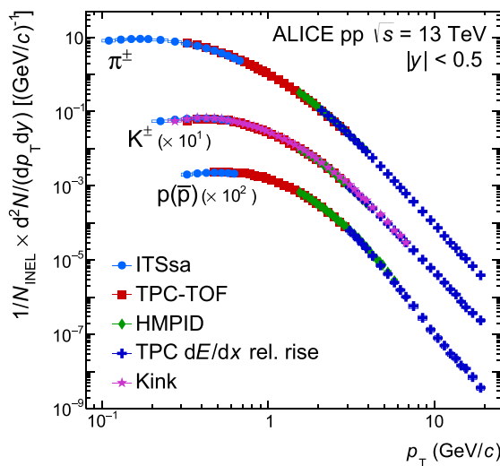
Fig. 3 Left panel: p_T spectra of \pi^\pm , K^\pm , and p(\bar{p}) measured at midrapidity ( |y| < 0.5 ) in pp collisions at \sqrt{s} = 13 \text{ TeV} using different PID techniques. The spectra are normalized to the number of inelastic collisions. Right panel: The ratios of individual spectra to the com-
