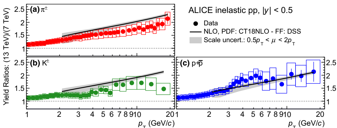
Fig. 18 Ratios of transverse-momentum spectra of \pi^\pm , K^\pm , and p(\bar{p}) in minimum bias inelastic pp collisions at \sqrt{s} = 13 TeV to those at \sqrt{s} = 7 TeV [25]. Solid lines show predictions from a next-to-
