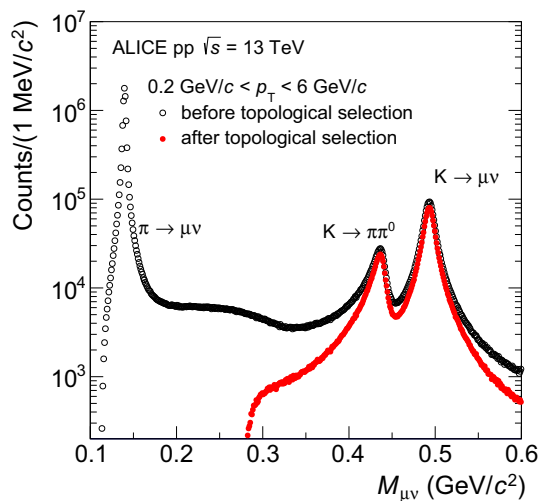
Fig. 2 Kink invariant mass distribution for charge summed particles in the mother particle transverse momentum interval 0.2 \text{ GeV}/c < p_T < 6 \text{ GeV}/c , before (open circle) and after (full circle) topological selections
