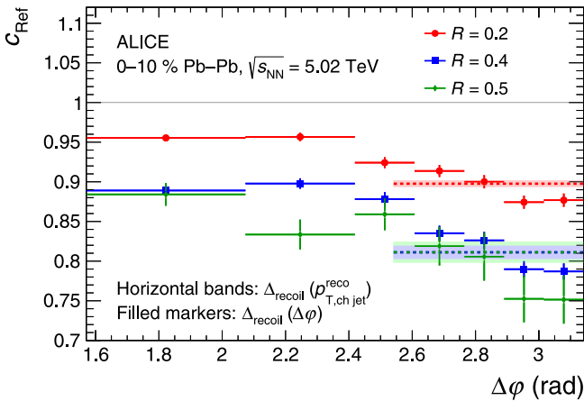
FIG. 5. Scaling factor c_{\text{Ref}} of \Delta_{\text{recoil}}(\Delta\varphi) for R = 0.2, 0.4 , and 0.5 . The vertical bars indicate the statistical uncertainties. The value of c_{\text{Ref}} for the \Delta_{\text{recoil}}(p_{T,\text{jet}}^{\text{reco}}) analysis, which integrates over the region |\Delta\varphi - \pi| < 0.6 , is displayed as a horizontal bar for each value of R , with shaded bands indicating statistical uncertainty.
