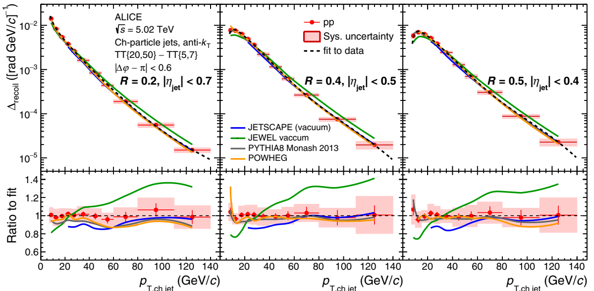
FIG. 11. (upper panels) corrected \Delta_{\text{recoil}}(p_{T, \text{ch jet}}) distributions measured for R = 0.2 (left), 0.4 (middle), and 0.5 (right) in pp collisions at \sqrt{s} = 5.02 TeV, compared with calculations from JETSCAPE [110], JEWEL [115,116], PYTHIA8 [99,100], and POWHEG [102–105]. (lower panels) Ratio of the data and calculations to a functional fit of the measured \Delta_{\text{recoil}}(p_{T, \text{ch jet}}) distributions.
