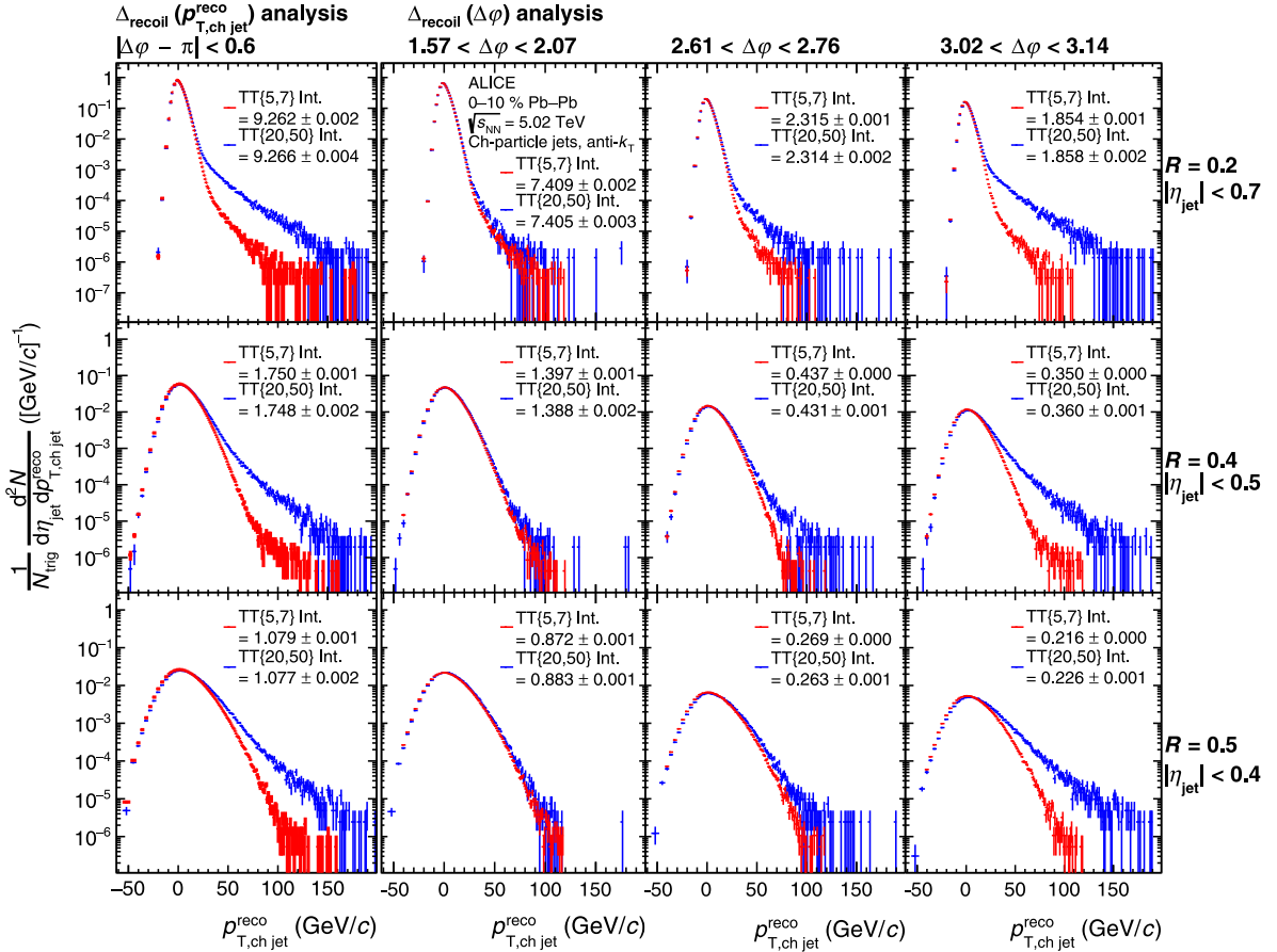
FIG. 3. Trigger-normalized semi-inclusive recoil jet distributions for \text{TT}_{\text{sig}} - and \text{TT}_{\text{ref}} -selected populations in central Pb-Pb collisions at \sqrt{s_{\text{NN}}} = 5.02 TeV, for R = 0.2 (upper panels), 0.4 (middle panels), and 0.5 (lower panels). The \Delta\rho correction (Sec. IV A) has been applied to the \text{TT}_{\text{ref}} distributions. The left column shows distributions in the \Delta\phi acceptance of the \Delta_{\text{recoil}}(p_{T,\text{jet}}) analysis. The remaining columns show distributions in selected \Delta\phi bins for the \Delta_{\text{recoil}}(\Delta\phi) analysis, with the second column having the largest deviation from \Delta\phi = \pi and the rightmost column at \Delta\phi \approx \pi .
