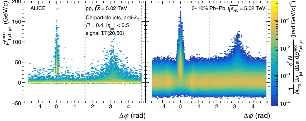
FIG. 1. Trigger-normalized recoil jet distributions ( R = 0.4 ) as a function of \Delta\phi and p_{T,\text{ch jet}}^{\text{reco}} , in pp collisions (left) and in Pb-Pb collisions (right) at \sqrt{s_{\text{NN}}} = 5.02 TeV, for \text{TT}\{20, 50\} GeV/c. The azimuthal region of the analysis is indicated by the vertical dashed lines.
