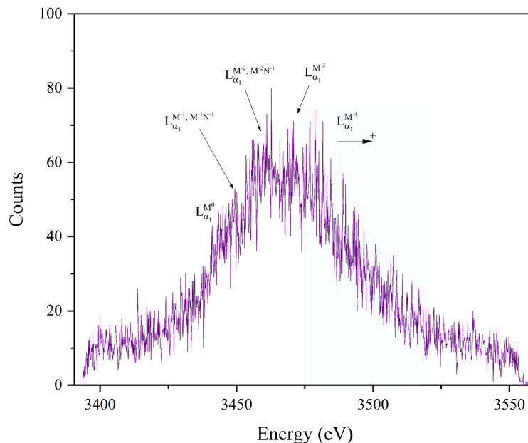
Figure 4.32. Sn L\alpha line due to 8 MeV \text{Si}^{4+} impact
