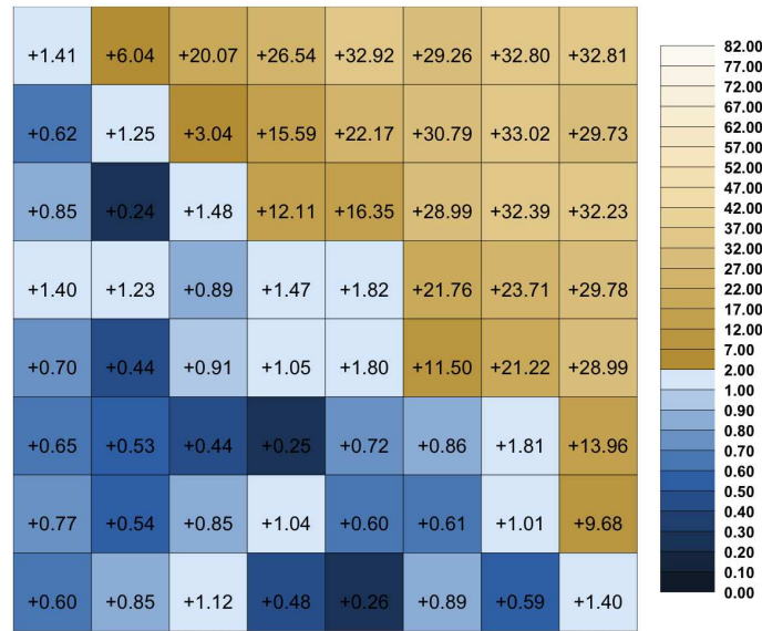
Figure 5.3: Simulation results for the perimeter process – \boldsymbol{\mu}^{(1)} = (100, 0) , \boldsymbol{\mu}^{(2)} = (0, 0) .
