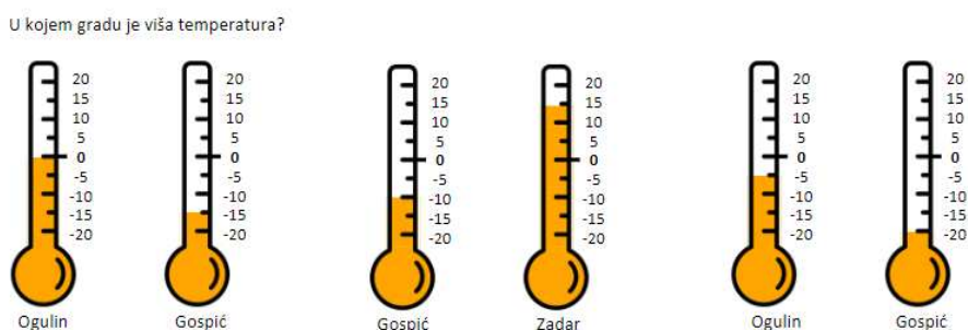
Slika 1.3: Model temperature
