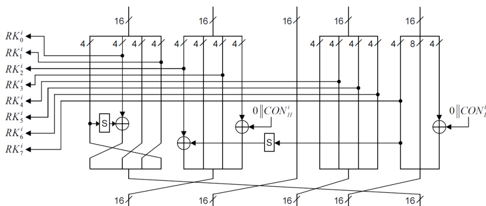
Slika 3.17: Twine Key Schedule [23]
