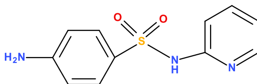
Slika 11. Sulfapiridin, \text{C}_{11}\text{H}_{11}\text{N}_3\text{O}_2\text{S} .
