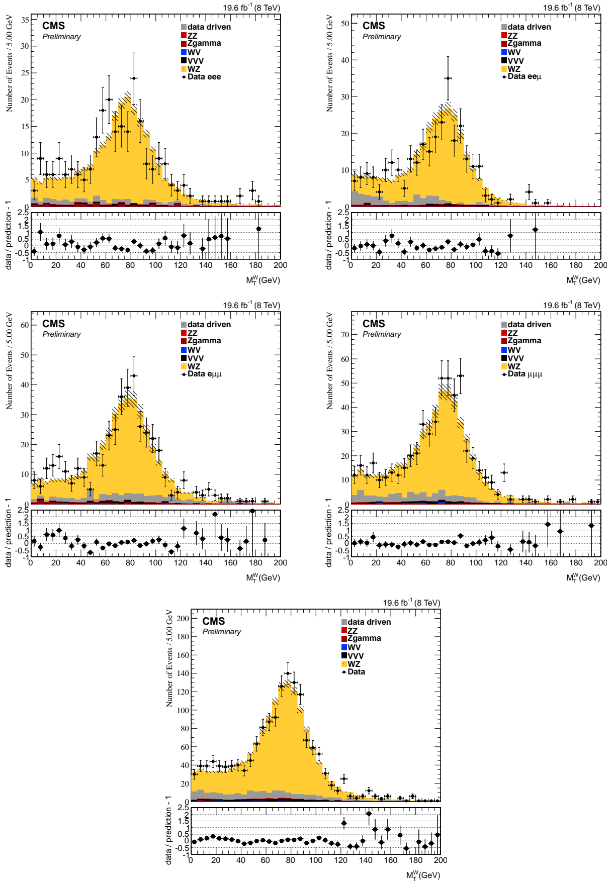
Figure 5.10: W transverse mass after final selection for 3e (first row left), 2e1\mu (first row right), 1e2\mu (second row left) and 3\mu (second row right) channels, and combination of all channels (third row).
