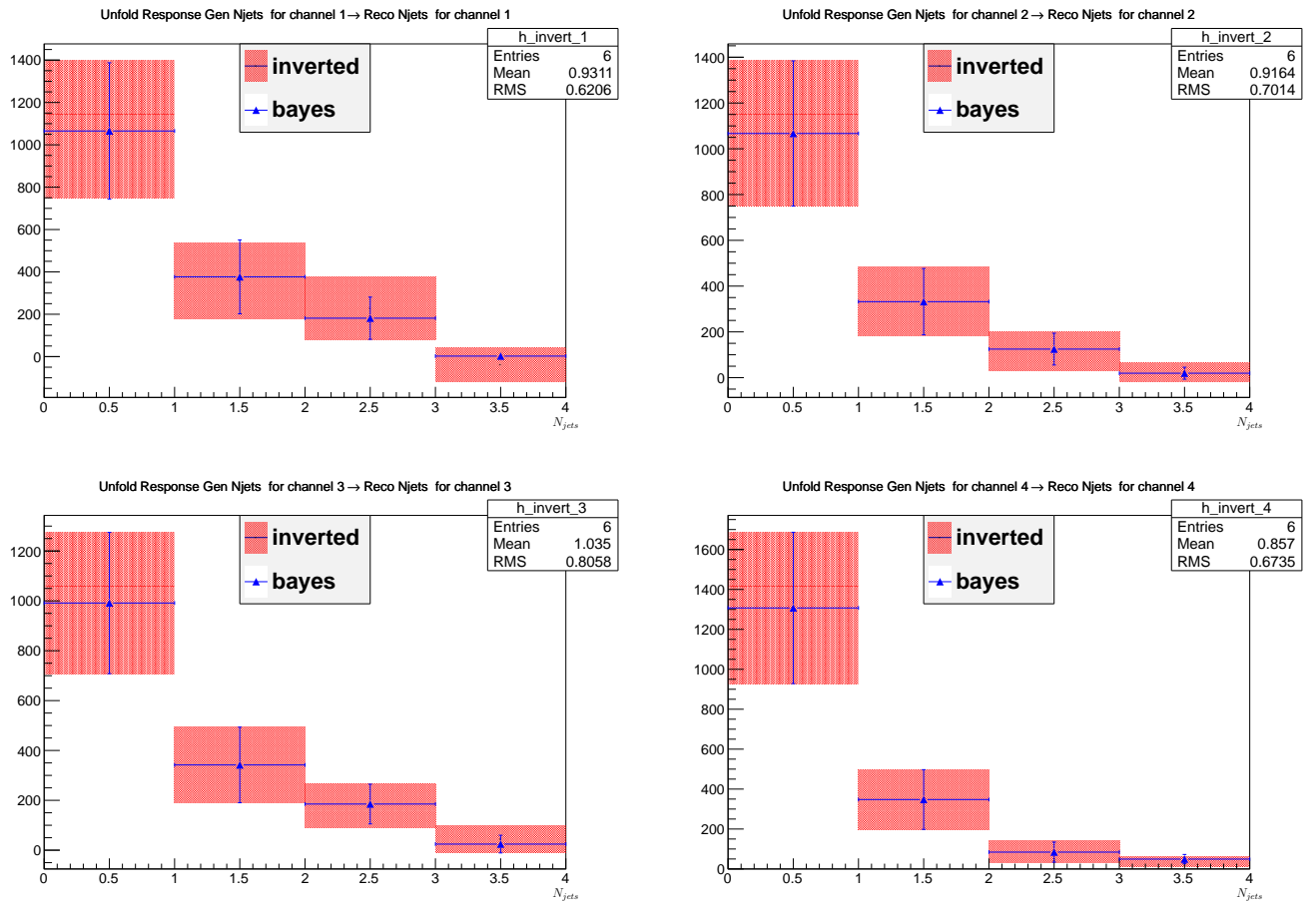
Figure 7.20: Comparison between Bayes unfolding algorithm and inversion for number of jets variable. Upper left plot corresponds to 3 electron channel, than 2 electrons and 1 muon (upper right), 1 electron and 2 muons (down left) and 3 muons (down right)
