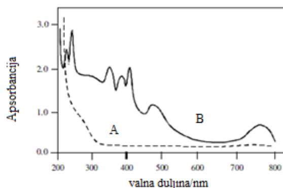
Slika 29: Apsorpcijski spektar 2 \times 10^{-4} \text{ mol L}^{-1} otopine \text{NH}_4\text{VO}_3 (A) i 1 \times 10^{-4} \text{ mol L}^{-1} otopine \text{NH}_4\text{VO}_3 u prisutstvu 2 \times 10^{-4} \text{ mol L}^{-1} otopine NA (B)
