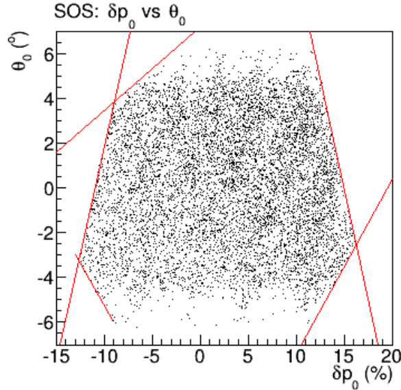
Figure 6.21 — SOS target coordinates \delta p_0 vs. \theta_0 . Cuts on SOS acceptance are represented by red lines.
