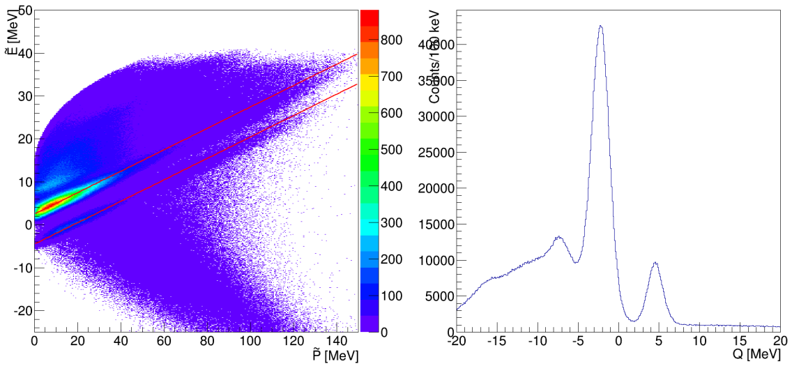
Figure 4.34: Left: The Catania plot for the {}^9\text{Be}({}^{13}\text{C}, {}^{14}\text{C } {}^4\text{He}) reaction, {}^4\text{He} detected in the T1 and {}^{14}\text{C} in the T2. The two red lines are denoting the position of reaction loci for the undetected {}^4\text{He} : the lowest for all nuclei in the ground state and the second one for the reaction channel with the {}^{14}\text{C}(E_x = 7 \text{ MeV}) . The lines were shifted by +2.0 MeV to reproduce the data. Right: The corresponding Q -value spectrum.
