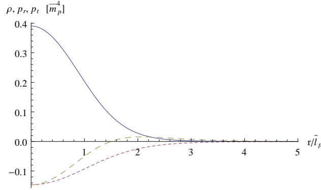
Figure 3.7. The energy density (solid curve), radial (short-dashed curve) and transverse pressure (long-dashed curve) for \xi = -0.9 , \lambda_\phi = -30 , \sigma_0 = 0.26 . Also m_\phi^2 = \bar{m}_P^2 .
