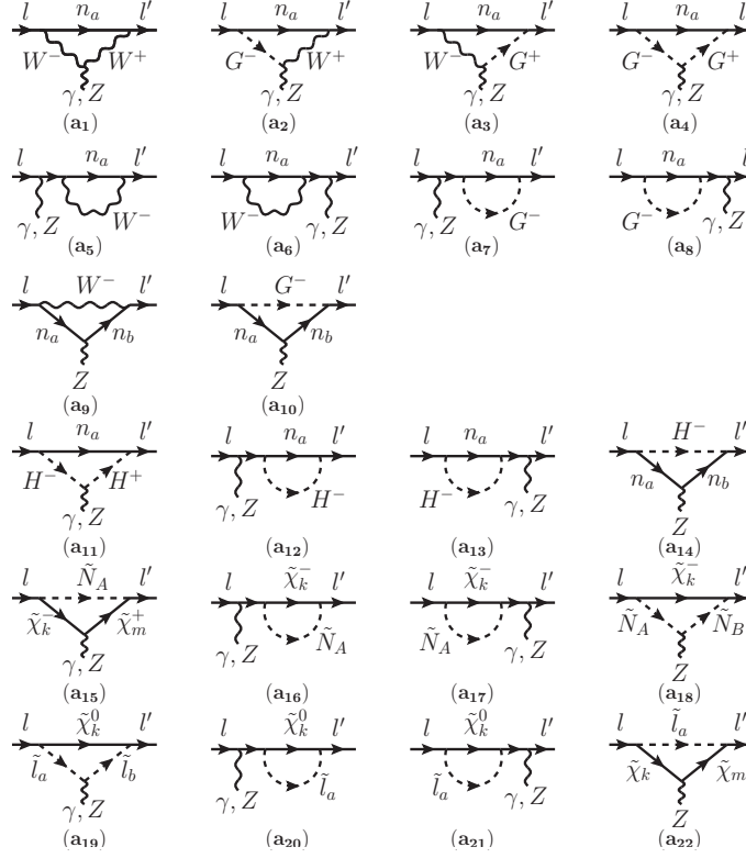
Figure 3.1: Feynman graphs contributing to l \rightarrow l'\gamma and Z \rightarrow l^C l' ( l \rightarrow Z l' ) amplitudes. Here n_a ( a = 1 \dots 6 ) and \tilde{N}_A ( A = 1 \dots 12 ) stand for neutrinos and sneutrinos in mass basis, respectively.
