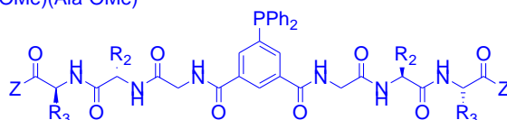
B3a , Lig-(Gly-Val-Phe-OMe) 2 B3b , Lig-(Gly-Pro-Phe-OMe) 2
