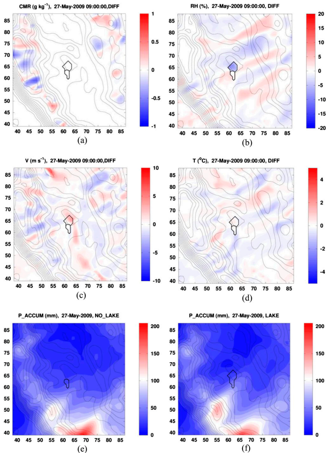
FIG. 7. As in Fig. 4, but for the SC at 0900 UTC 27 May 2009.
