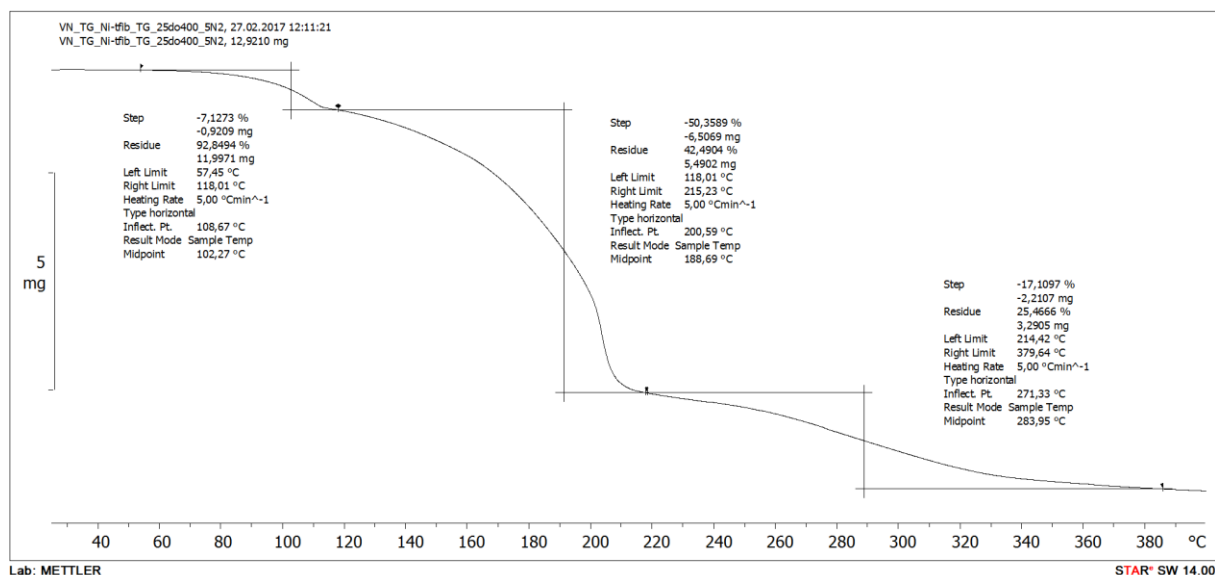
Slika D46. TG krivulja kokristala [\text{Ni}(\text{acac})_2(\text{H}_2\text{O})_2](1,4\text{-tfib}) .
