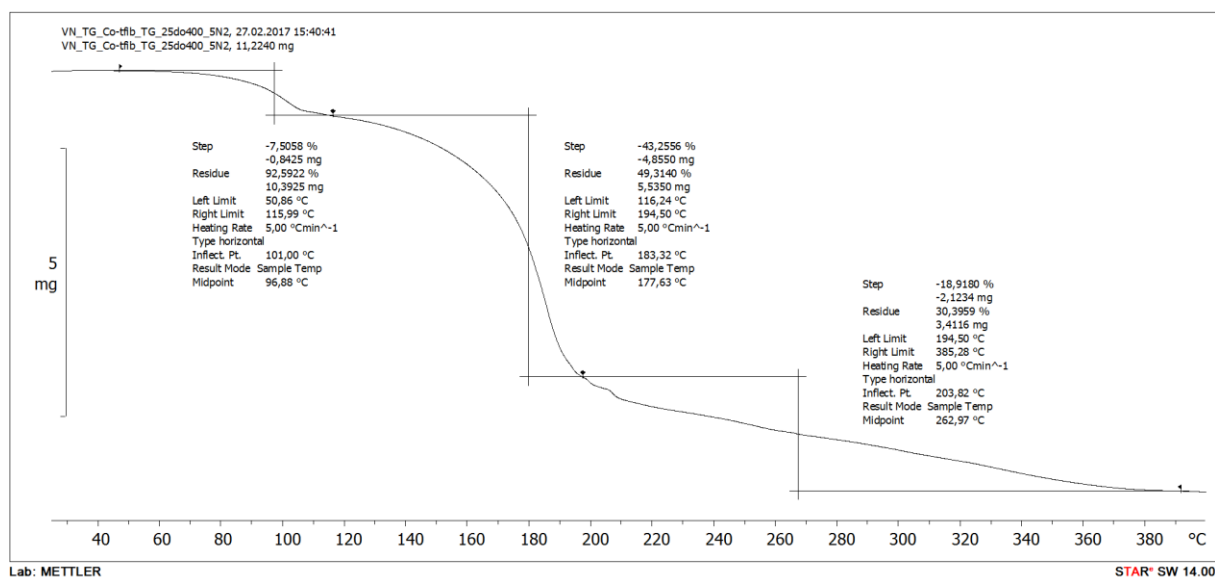
Slika D45. TG krivulja kokristala [\text{Co}(\text{acac})_2(\text{H}_2\text{O})_2](1,4\text{-tfib}) .
