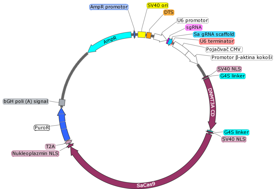
pN-DNMT3a/SaCas9/Puro/sgRNA 8539 bp
