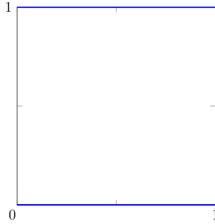
Figure 3.1: The graph of f in Example 3.29
