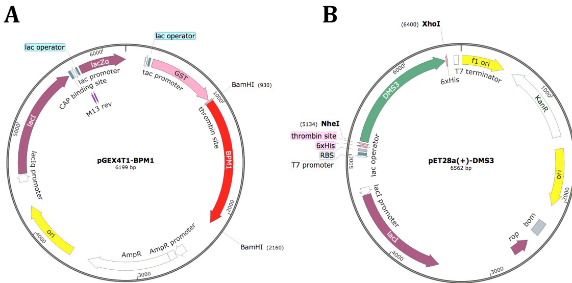
Figure 3. Plasmid maps of pGEX4T1-BPM1 (A) and pET28a(+)-DMS3 (Lorković et al., 2012) (B) used for BPM1 and DMS3 protein expression respectively. Apart from a selection marker, an ori site for plasmid replication and a multiple cloning site (MCS), expression plasmids also contain sequences for a protein tag (GST or 6× His), a strong inducible promoter and a regulatory region upstream of the MCS, a transcription terminator and lacI gene which encodes a repressor protein.
