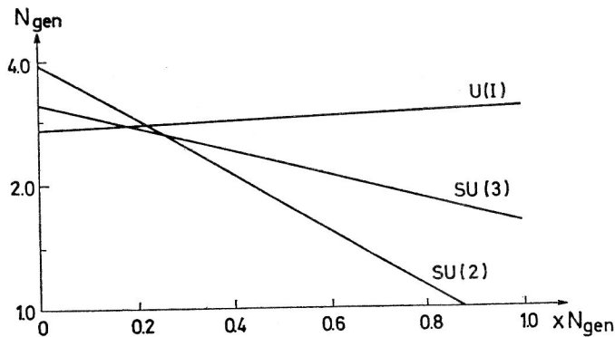
Fig. 4. Interaction of the three lines corresponding to the three gauge couplings, as given by Eqs. (14) and (15).
