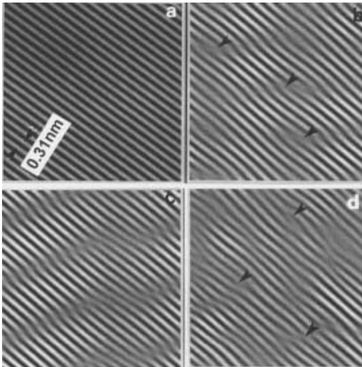
Figure 9. Refinement in overlapping layers L. Filtered lattice images with spots 7 ( 7_1, 7_2, 7_3 ): (\bar{1}11) m -ZrO 2 , (222) Y 2 O 3 , (\bar{1}11) m -ZrO 2 from FT of Figure 8(j) with different filtering mask radii: (a) (\bar{1}11) m -ZrO 2 ( d = 0.316 nm), one pixel; (b) all spots 7, three pixel; (c) two spots 7_1 and 7_2 , isolated with one pixel mask; (d) five pixels encircling all three spots 7.
