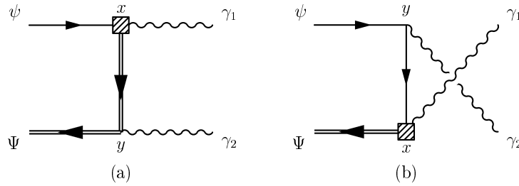
Fig. 3. The shaded boxes indicate the combination of the unrotated off-shell transition (proportional to B_F ) and the on-shell magnetic moment transition (proportional to B_\sigma ), giving the effective vertex in Eq. (47).
