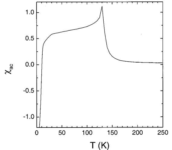
FIG. 1. Plot of the \text{RuSr}_2\text{EuCu}_2\text{O}_8 zero-field ac susceptibility against temperature for an ac field of 0.05 G and a frequency of 1 kHz. The susceptibility has not been corrected for demagnetization effects.
