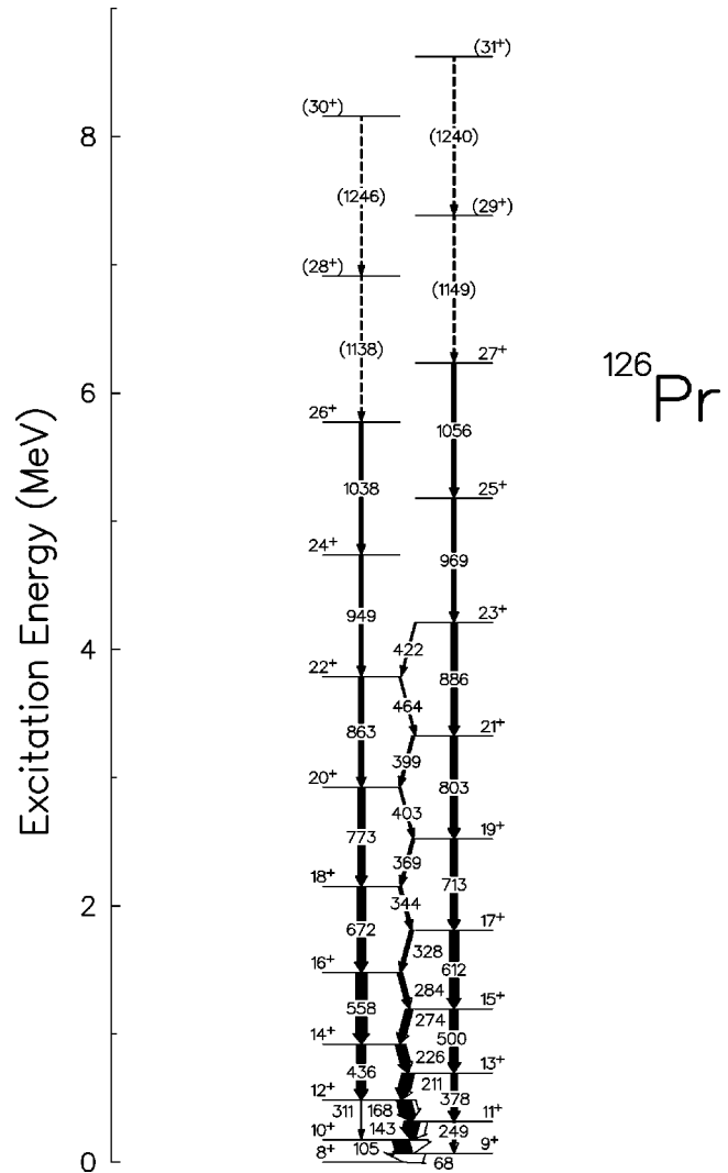
FIG. 4. Level scheme of ^{126}\text{Pr} deduced from the present work. The transition intensities are proportional to the width of the arrows.
