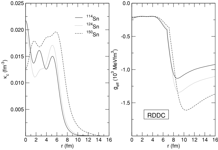
FIG. 7. The anomalous densities in ^{114}\text{Sn} , ^{124}\text{Sn} , ^{150}\text{Sn} isotopes as functions of the radial coordinate (left) and the density-dependent curves g_{\text{eff}} [Eq. (19)] (right). The calculations are performed with the renormalization of the density-dependent coupling Eq. (23) (RDDC).
