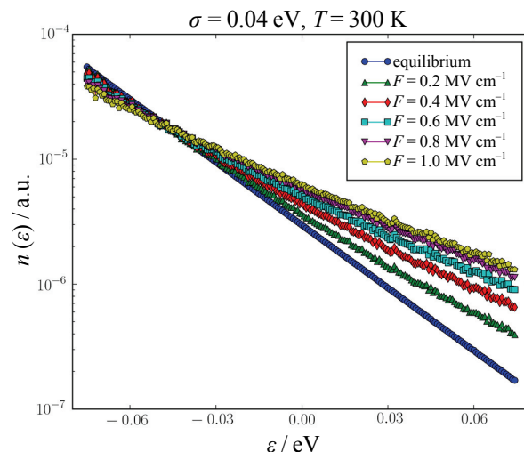
Figure 3. The mean occupancy n(\varepsilon) in the current-carrying state, with n(\varepsilon) numerically calculated through Eq. (16). Note the logarithmic scale on the vertical axis. The energy range shown in the figure covers the energies with reliable statistics. The data-set with the highest slope corresponds to the system in equilibrium at the temperature T , with the slope given by -1/T . The absolute value of the slope decreases as the strength of the applied electric field increases. This slope is identified as 1/T^* , with T^* > T , being the effective temperature of the system out of equilibrium.
