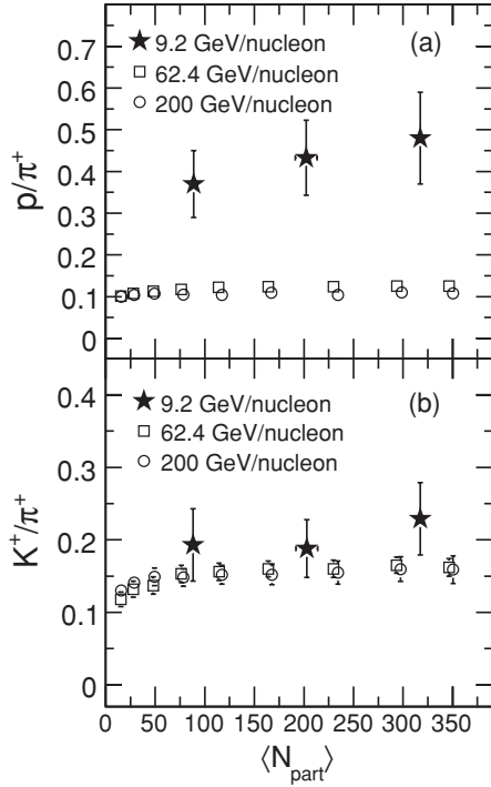
FIG. 15. Variation of (a) p/\pi^+ and (b) K^+/\pi^+ ratios as a function of \langle N_{\text{part}} \rangle for Au + Au collisions at \sqrt{s_{NN}} = 9.2 GeV. For comparison, we also show the corresponding results from Au + Au collisions at \sqrt{s_{NN}} = 62.4 and 200 GeV [4,23,37]. The errors shown are the quadrature sum of statistical and systematic uncertainties. The systematic errors for p/\pi^+ and K^+/\pi^+ for \sqrt{s_{NN}} = 9.2 GeV data are \sim 25\% and 22\% , respectively, and similar for all the collision centralities studied.
