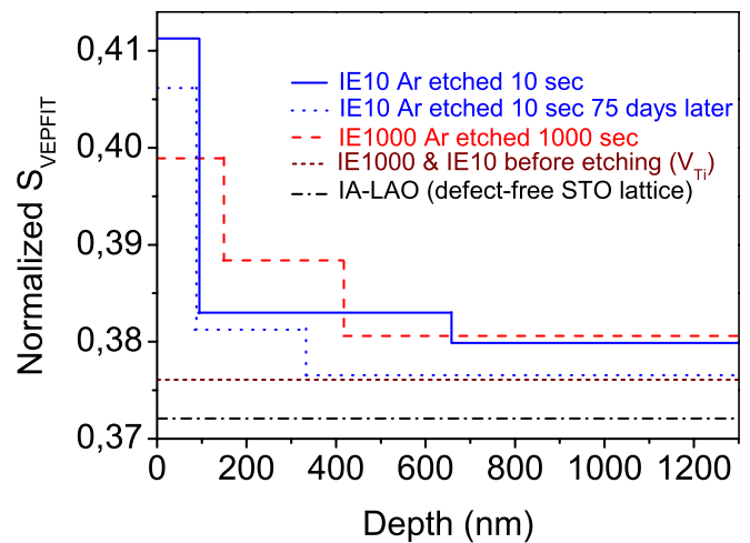
FIG. 5. (Color online) Depth profile of vacancy defects in ion-etched and as-received substrates probed by positrons in STO, extracted from VEPFIT spectra simulation.
