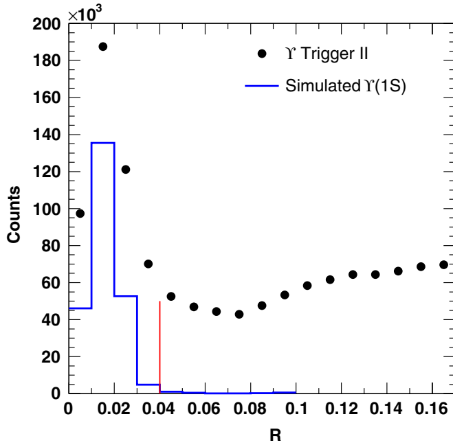
FIG. 8 (color online). The radial distance R = \sqrt{\Delta\eta^2 + \Delta\phi^2} between the TPC track and the EMC electron cluster for simulated \Upsilon daughters (line histogram, arbitrary scale), and the R distribution from data (circles). We reject candidate tracks with R > 0.04 (vertical line).
