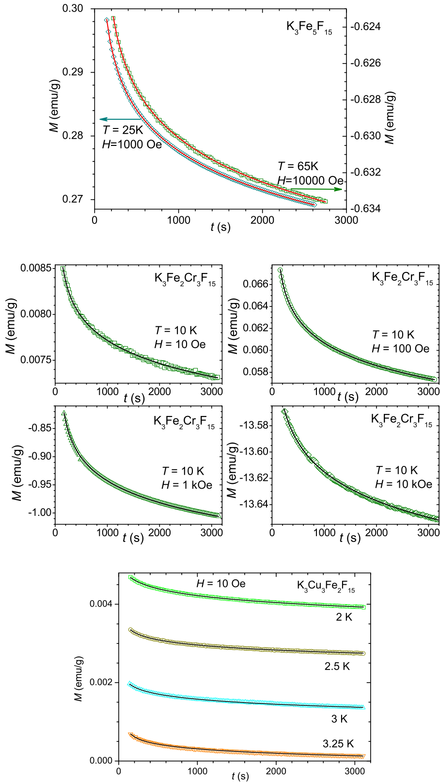
FIG. 2. Some typical magnetization relaxation curves of K_3Fe_5F_{15} (upper panel), K_3Fe_2Cr_3F_{15} (middle 4 panels), and K_3Cu_3Fe_2F_{15} (lower panel) after different magnetic field reversals from H to -H . Lines are the logarithmic fitting curves defined by Eq. (1).
