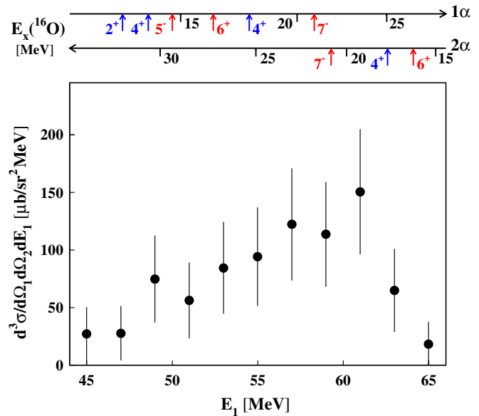
FIG. 1 (color online). The spectrum from the Letter [1], with additional axes giving the ^{16}\text{O} excitation energies in two \alpha - ^{12}\text{C} pairs. The arrows show the positions of the ^{16}\text{O} known members [2] of rotational bands with the ^{12}\text{C} + \alpha structure (red), and of the other states having large alpha-spectroscopic factor (blue).
